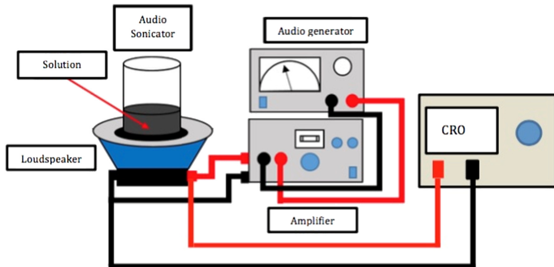
Fig. 3. The custom-made audiosonicator equipment design.
